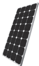
8x275w (2.2kW total) Mono Crystalline Solar Panels
